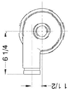
PLAN VIEW
